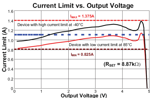
Fig.1 Current Limit Using 8.87k\Omega
